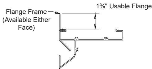
Flange Frame Available
